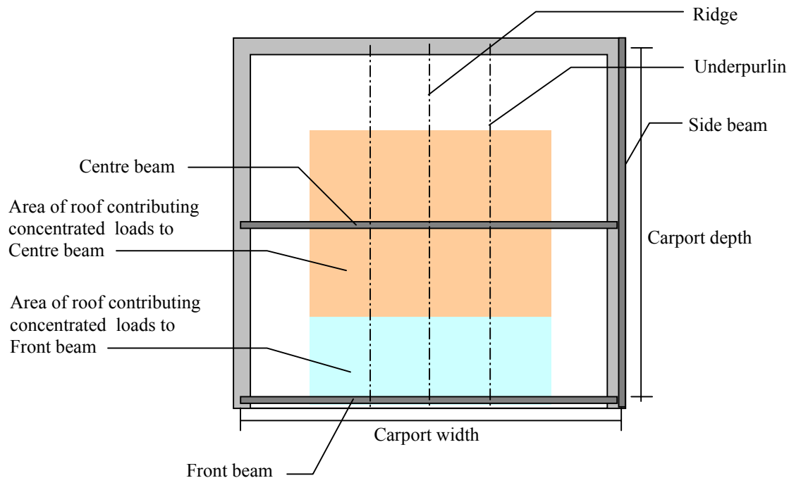
Figure 2 – Gable over Opening
